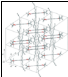
Fig. 2. A view of a 2x2x2 array of unit cells showing the coplanar fluorene units and the perpendicular octyl groups. Hydrogen atoms are omitted for clarity.
